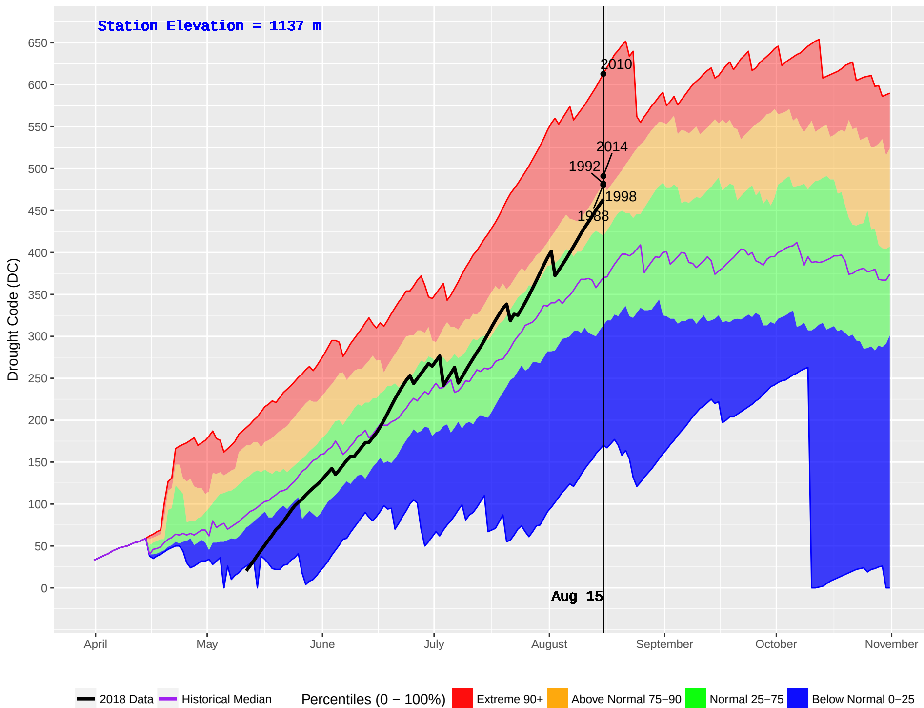
KLUSKUS (166) : Historical (1982–2016) and Current (2018) Daily Drought Code (DC)
