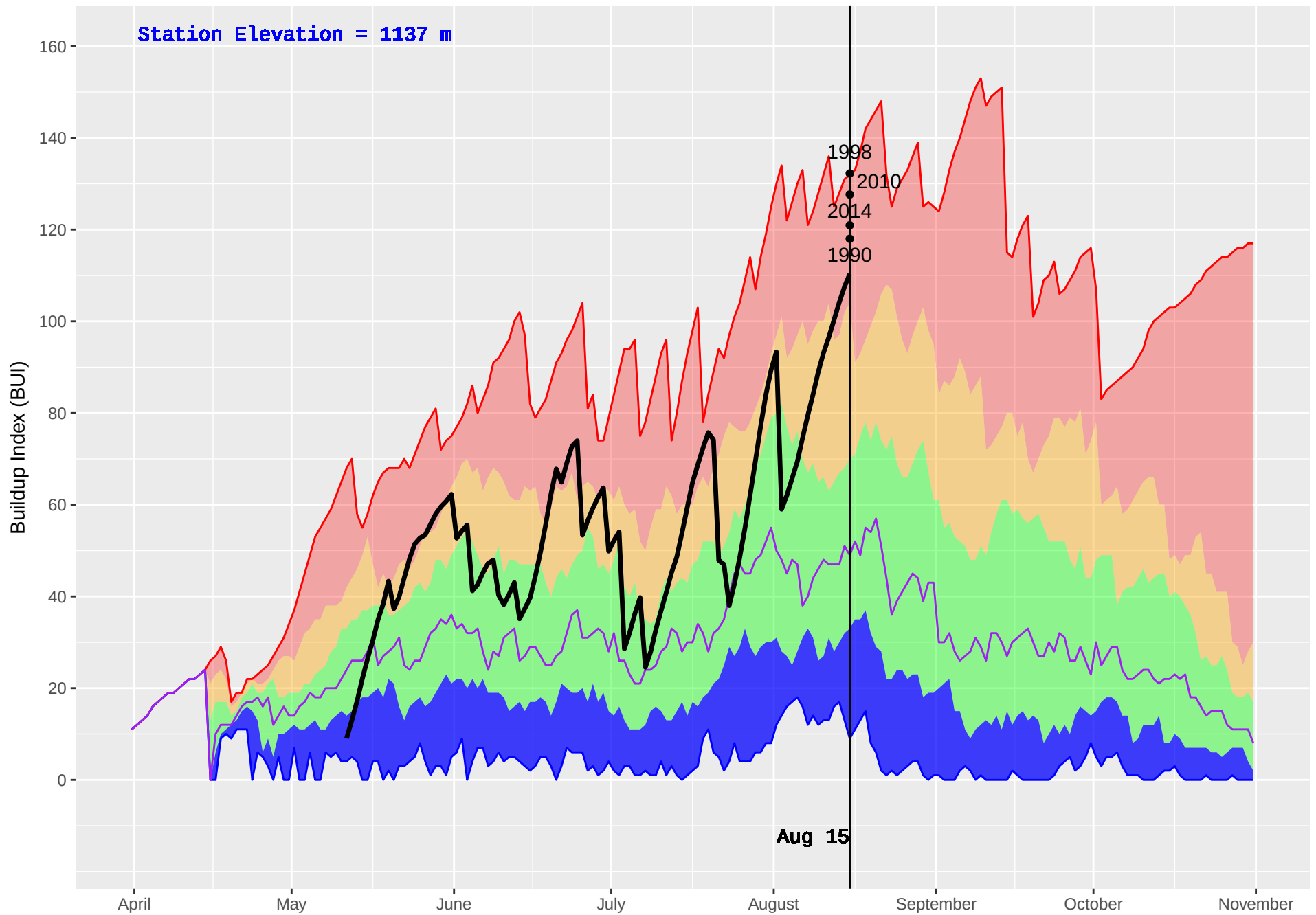
KLUSKUS (166) : Historical (1982–2016) and Current (2018) Daily Buildup Index (BUI)
